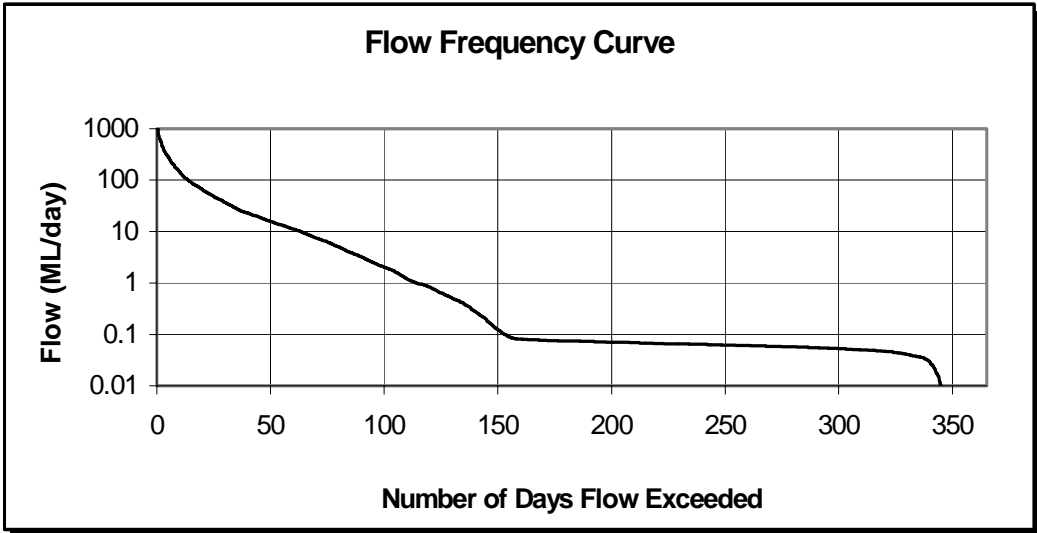
Figure 6. Daily Flow Frequency Curve – Cambrai
